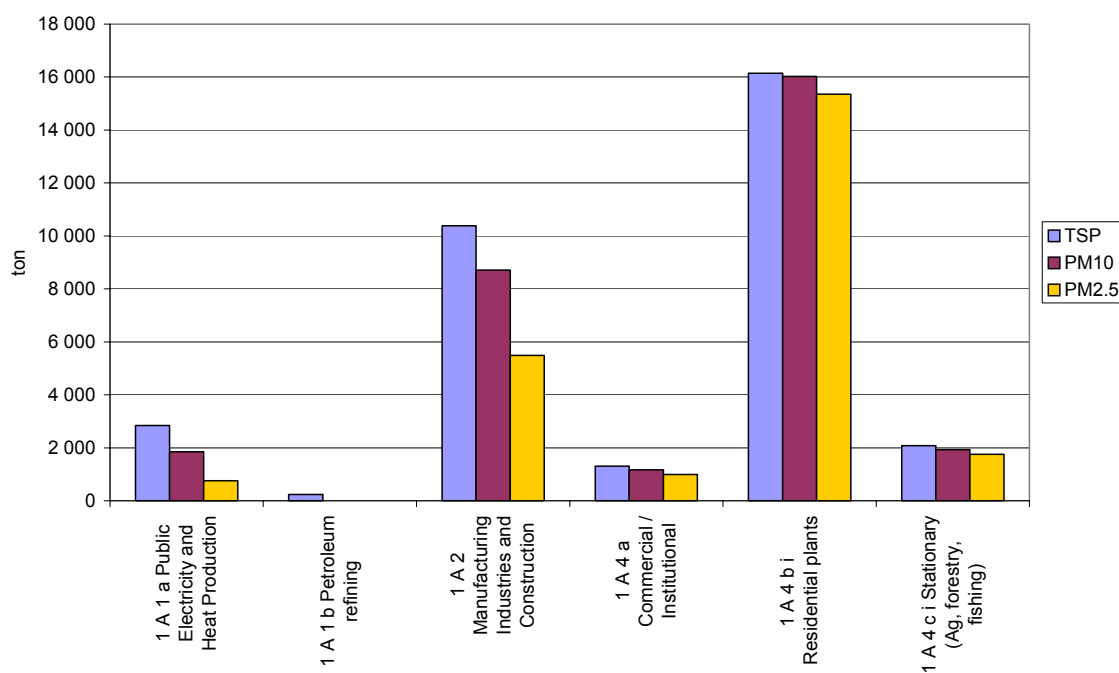
Figure 1. Annual PM emissions from stationary combustion in Denmark in 2000. The data are official inventory results from table IV 1A of the national emission as defined by Draft Guidelines for Estimating and Reporting Emissions Data (UNECE, 2002).
