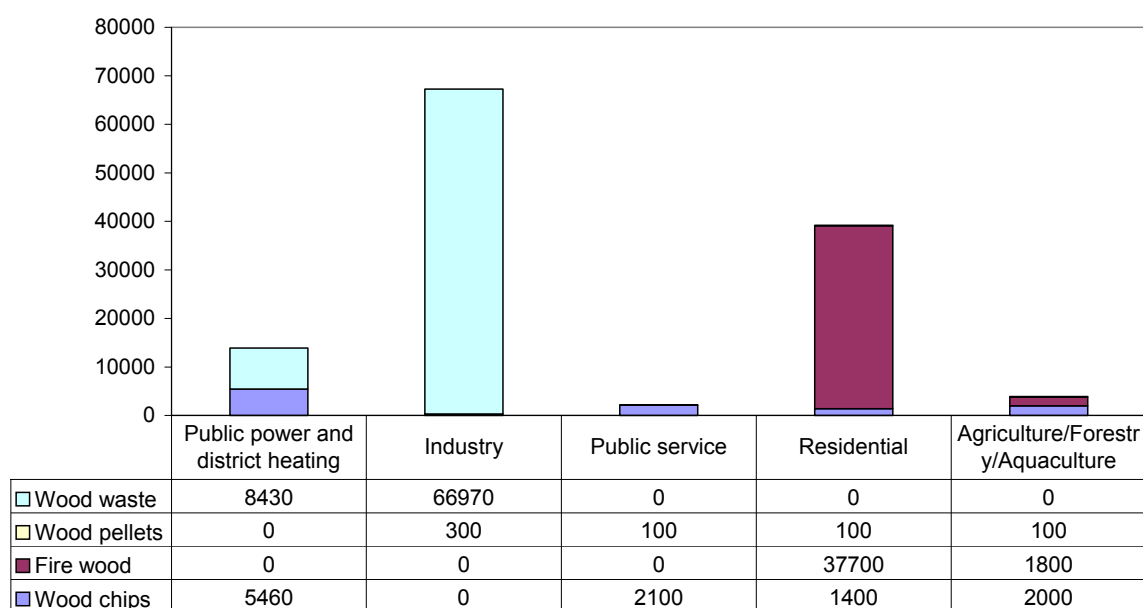
Figure 8. Wooden fuel consumption in TJ/year of wood chips, firewood, wood pellets and wood waste in different sectors in Finland in 2000.
