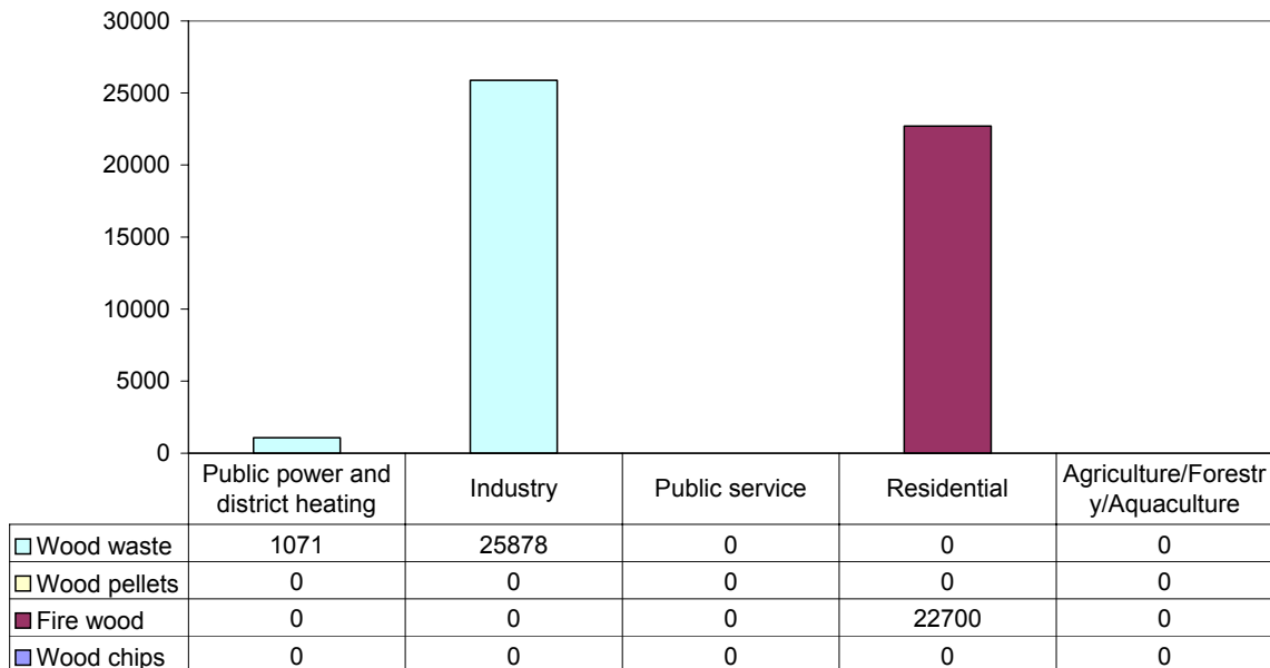
Figure 9. Wooden fuel consumption in TJ/year of wood chips, firewood, wood pellets and wood waste, different sectors in Norway in 2000.
