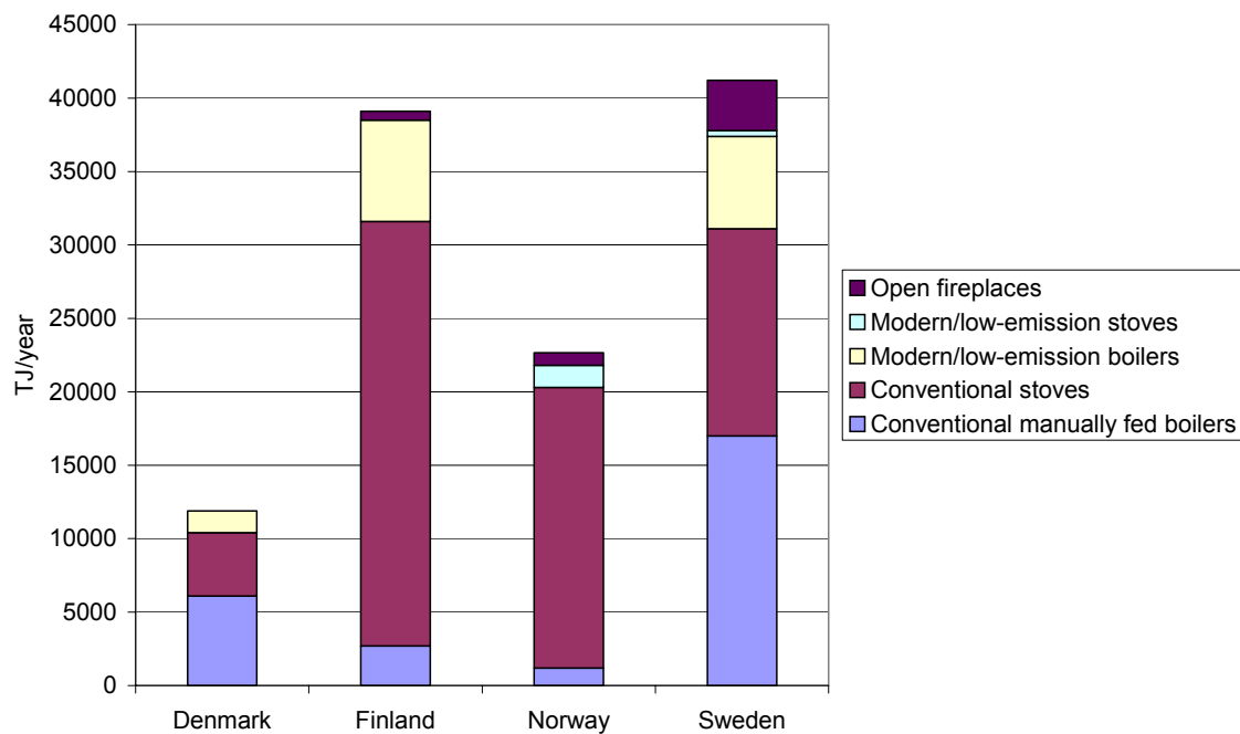
Figure 6. Wooden fuel use, total and in different combustion equipment in the Nordic countries in the residential sector (TJ/year, see explanations in Table 1).
