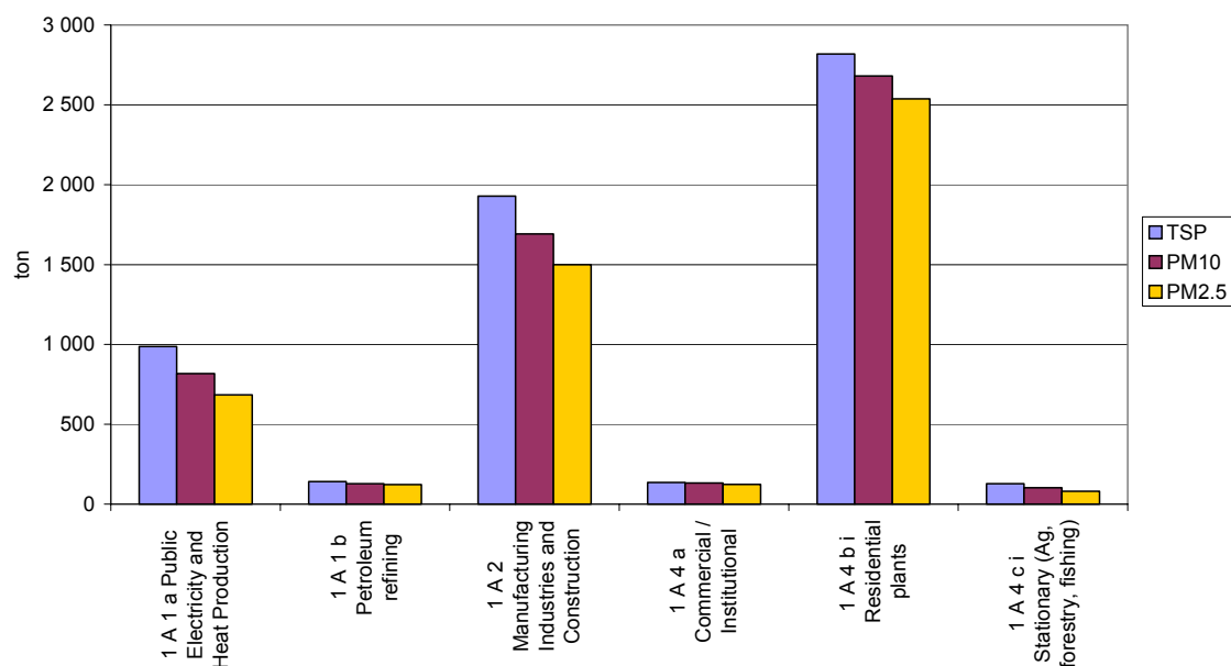
Figure 1. Annual PM emissions from stationary combustion in Denmark in 2000. The data are official inventory results from table IV 1A of the national emission as defined by Draft Guidelines for Estimating and Reporting Emissions Data (UNECE, 2002).
