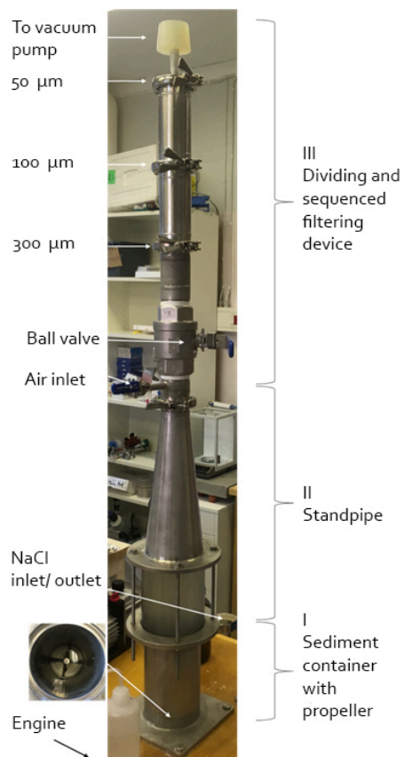
Figure A1: Schematic presentation of the density separation module for the extraction of anthropogenic micro particles from sediment. See text for detailed description on usage.
