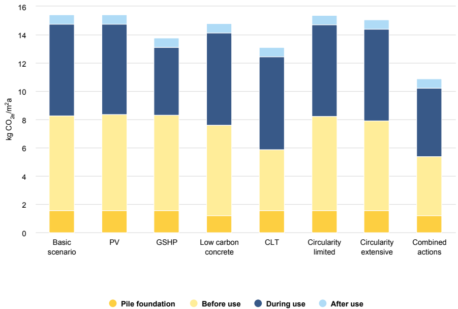
Figure 10. Building carbon footprint calculated for 50 years, for new construction with a foundation of 20 m steel-reinforced concrete piles.
