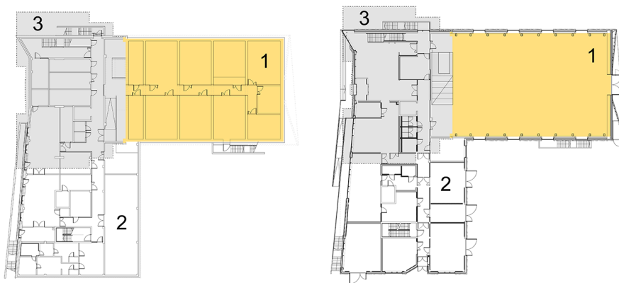
Figure 29. Basement (left) and the ground floor plan, Mäemaja building. The structures of the old test hall (1) were mainly preserved and spaces with poor functionality (3) demolished. New, larger office part (2) was constructed with a CLT timber frame.
