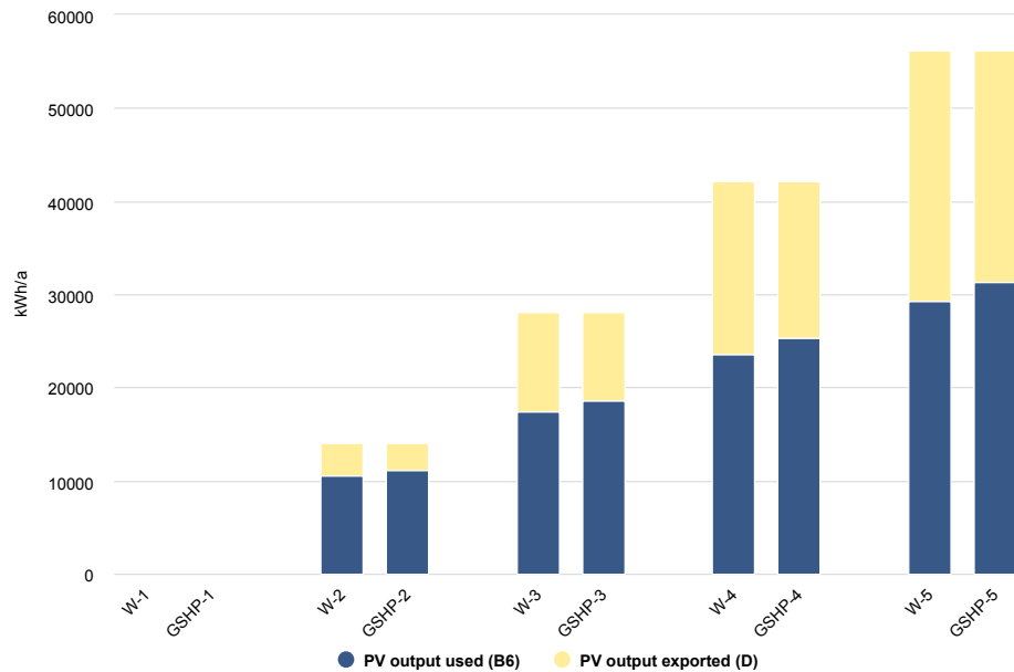
Figure 32. Photovoltaic system output, the shares of own use and export with district heating (left column) and GSHP (right column) and with various PV system dimensioning.
