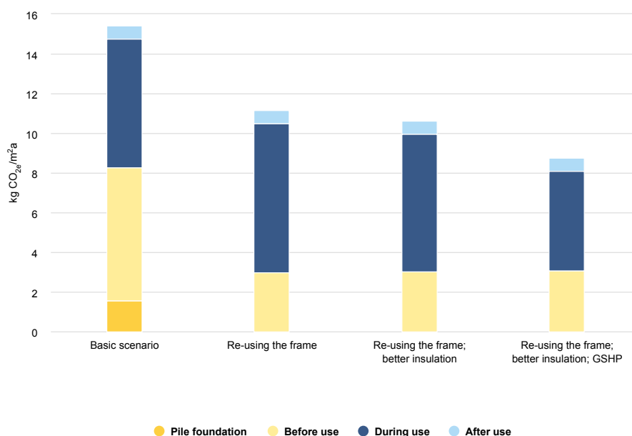
Figure 12. Building carbon footprint calculated for 50 years. Basic scenario is new construction with 20 m concrete piles, the other scenarios illustrate the effect from saving the building foundations and frame.
